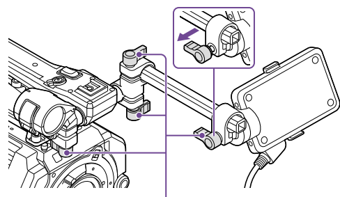
Clamp lever
